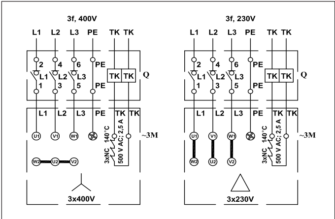
Wiring diagram No. 1*
